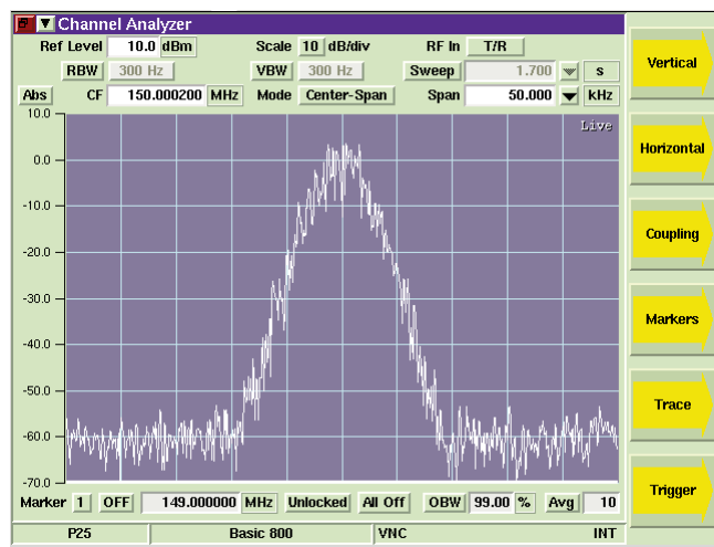
Spectrum Analyzer
